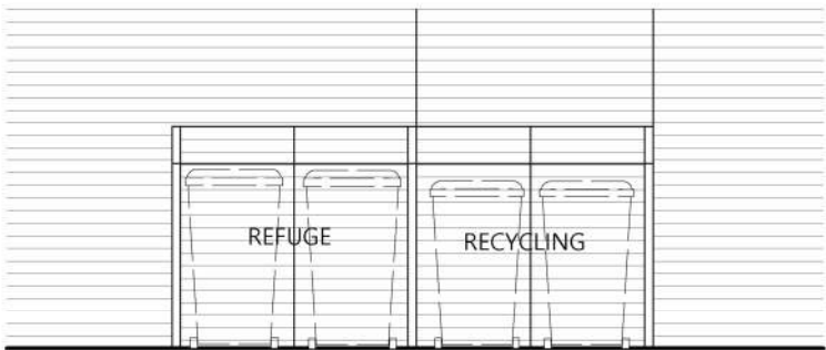
FRONT & SIDE ELEVATIONS OF REFUSE STORAGE FOR ALL FLATS
