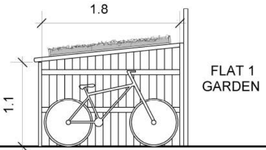
SECTION OF CYCLE STORAGE AREA FOR FLAT 1,2&3
